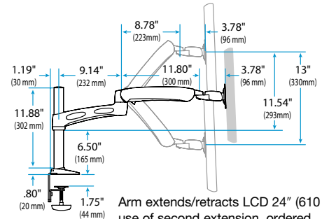
LCD rotates 90° portrait/landscape
